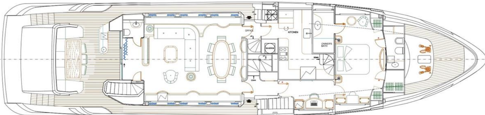
MAIN DECK
