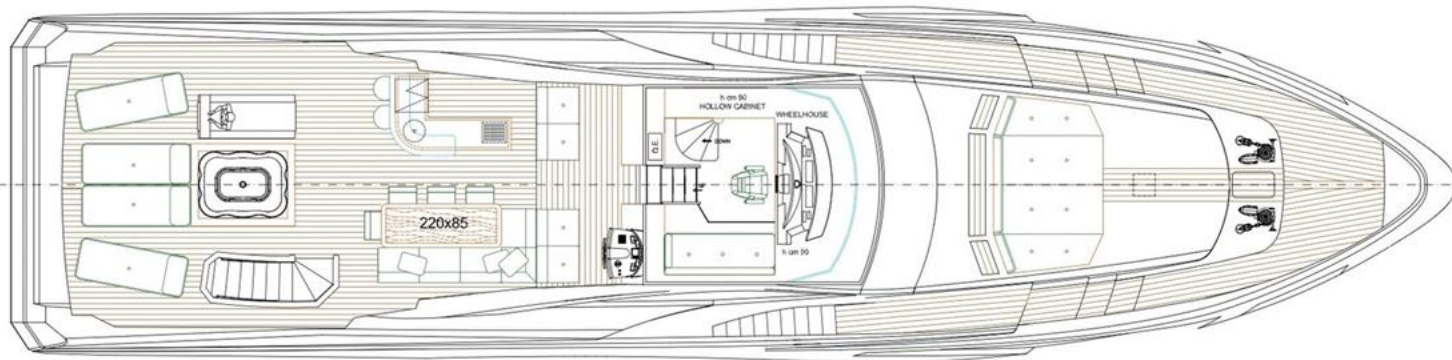
FLY DECK
